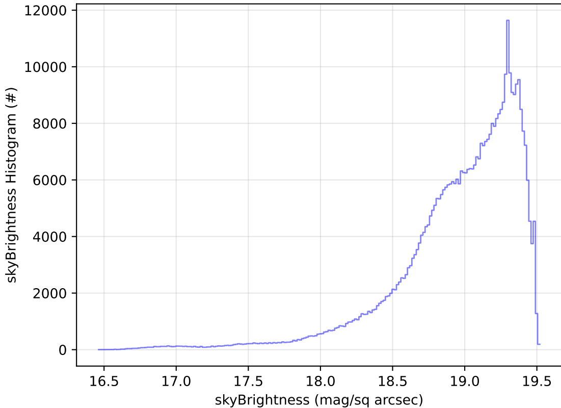
ddf_acor_sf30_lsf40_lsr10_v3.4_10yrs WFD z band: skyBrightness Histogram
