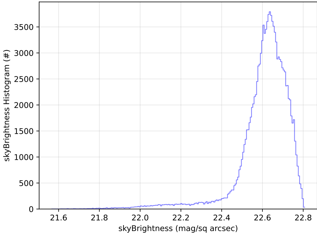
ddf_acor_sf30_lsf40_lsr10_v3.4_10yrs WFD u band: skyBrightness Histogram
