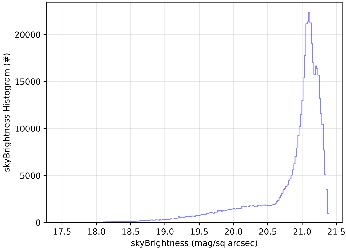
ddf_acor_sf30_lsf40_lsr10_v3.4_10yrs WFD r band: skyBrightness Histogram
