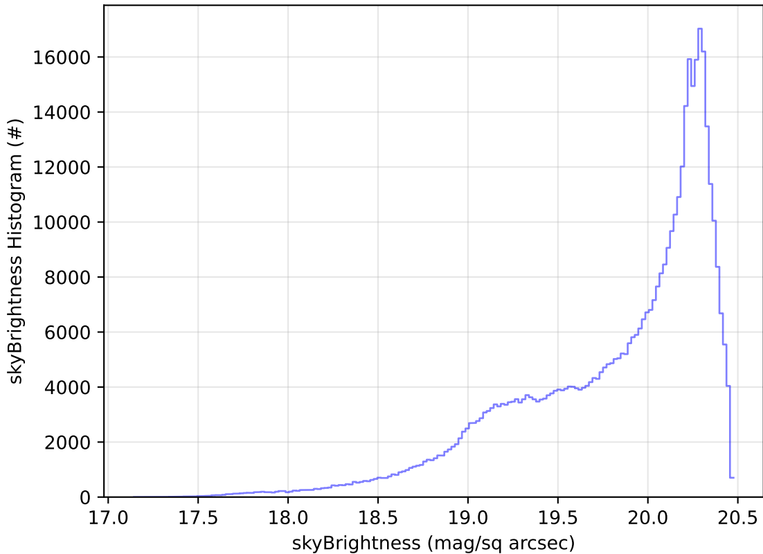
ddf_acor_sf30_lsf40_lsr10_v3.4_10yrs WFD i band: skyBrightness Histogram
