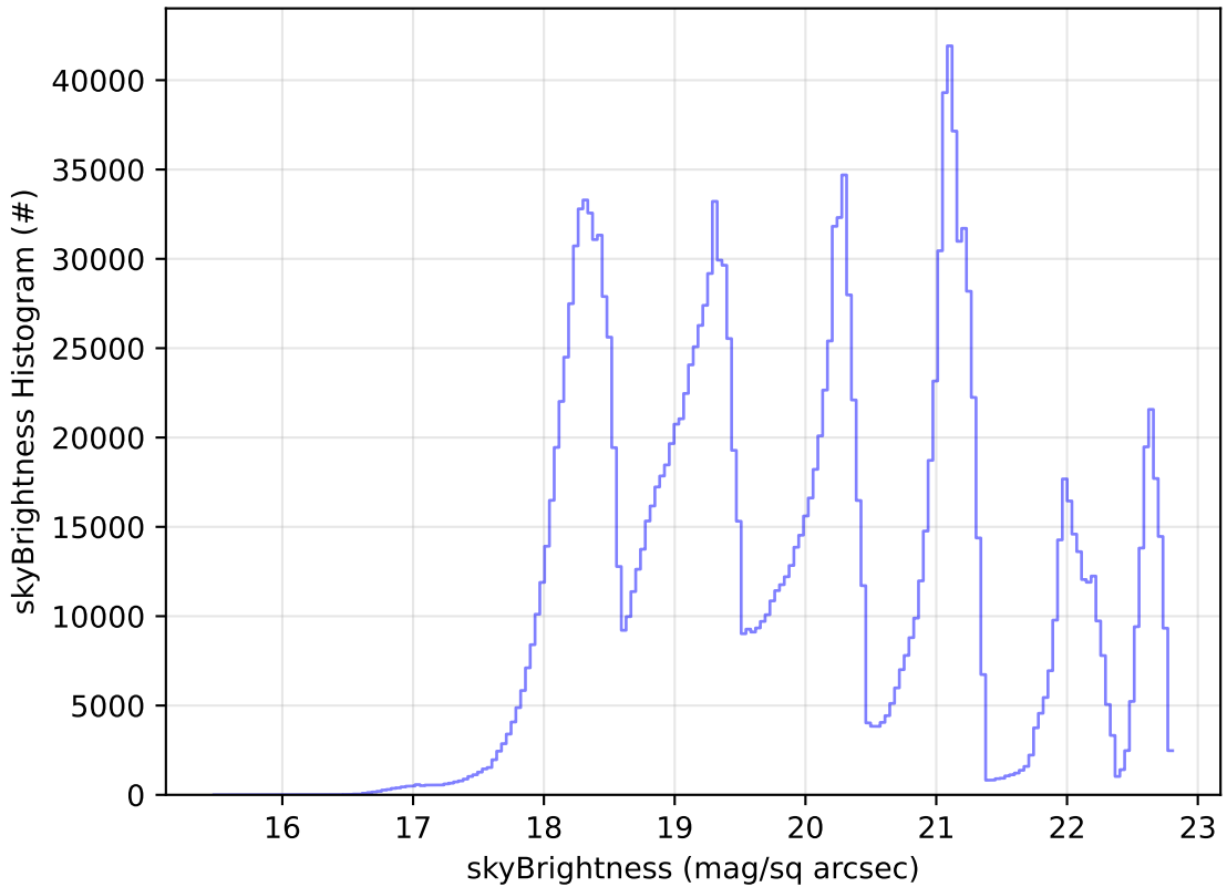
ddf_acor_sf30_lsf40_lsr10_v3.4_10yrs WFD all bands: skyBrightness Histogram
