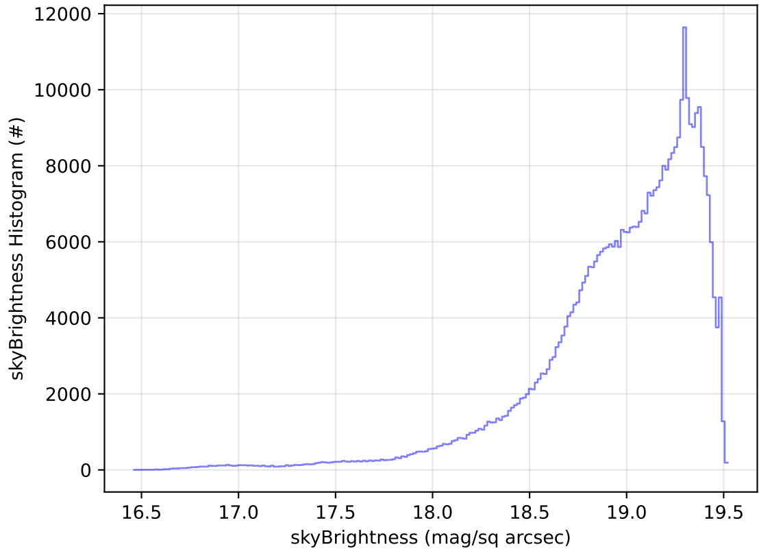
ddf_acor_sf30_lsf40_lsr10_v3.4_10yrs All sky z band: skyBrightness Histogram
