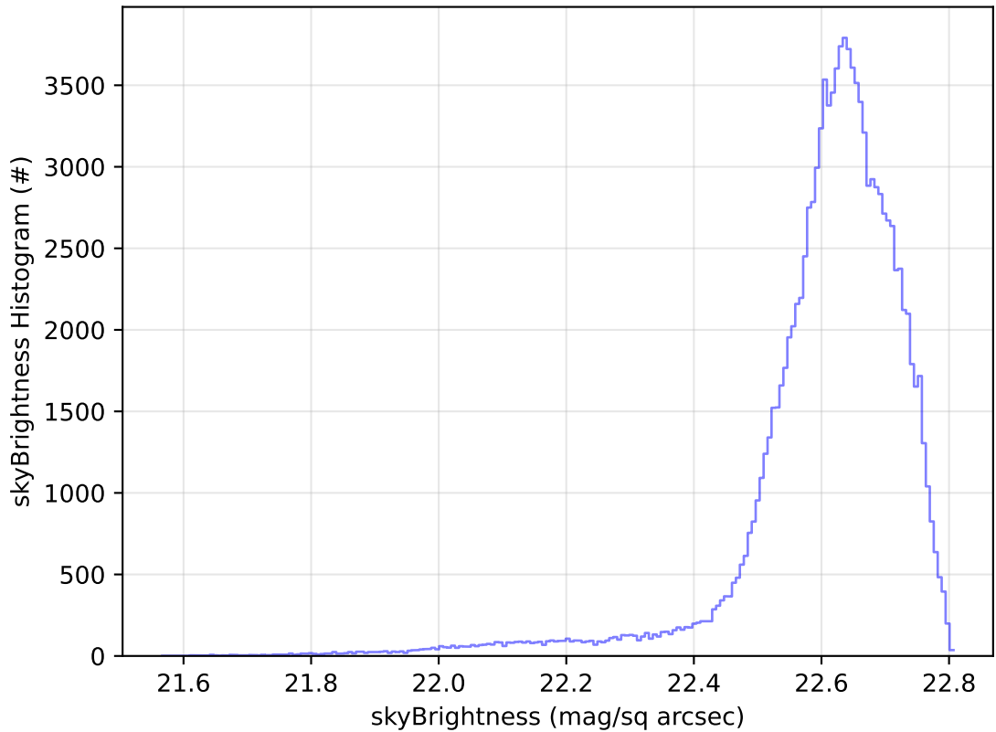
ddf_acor_sf30_lsf40_lsr10_v3.4_10yrs All sky u band: skyBrightness Histogram
