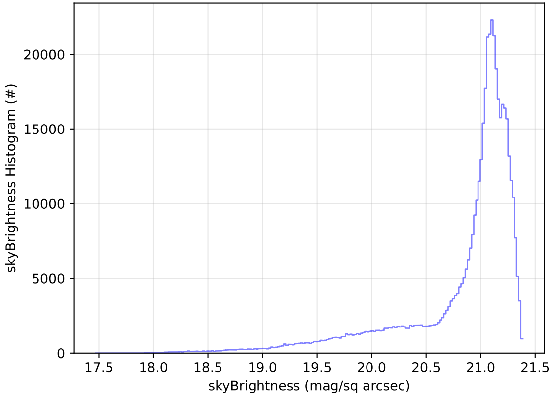
ddf_acor_sf30_lsf40_lsr10_v3.4_10yrs All sky r band: skyBrightness Histogram
