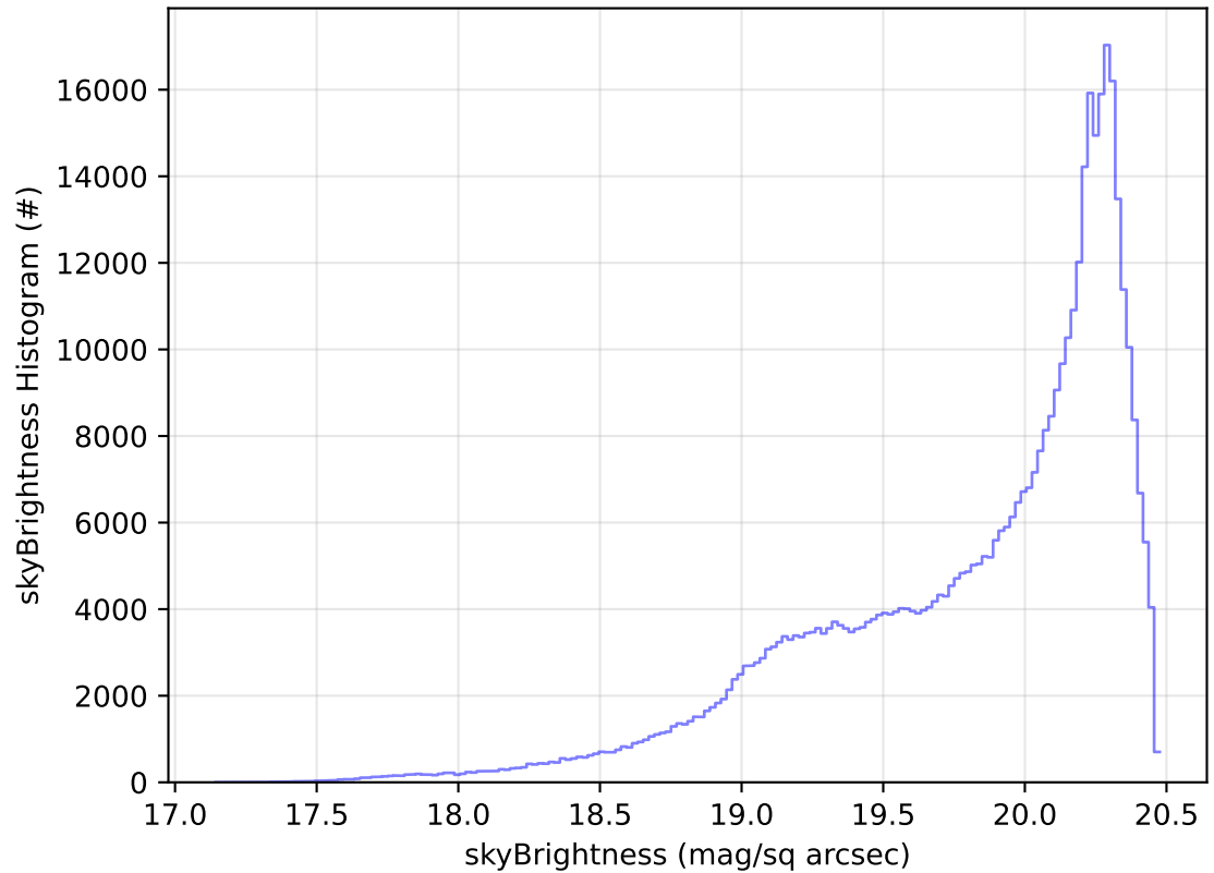
ddf_acor_sf30_lsf40_lsr10_v3.4_10yrs All sky i band: skyBrightness Histogram
