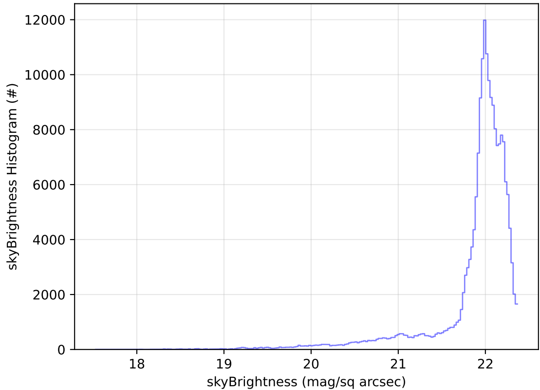
ddf_acor_sf30_lsf40_lsr10_v3.4_10yrs All sky g band: skyBrightness Histogram
