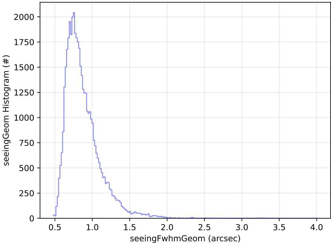
ddf_acor_sf30_lsf40_lsr10_v3.4_10yrs Yr 1 z band: seeingGeom Histogram
