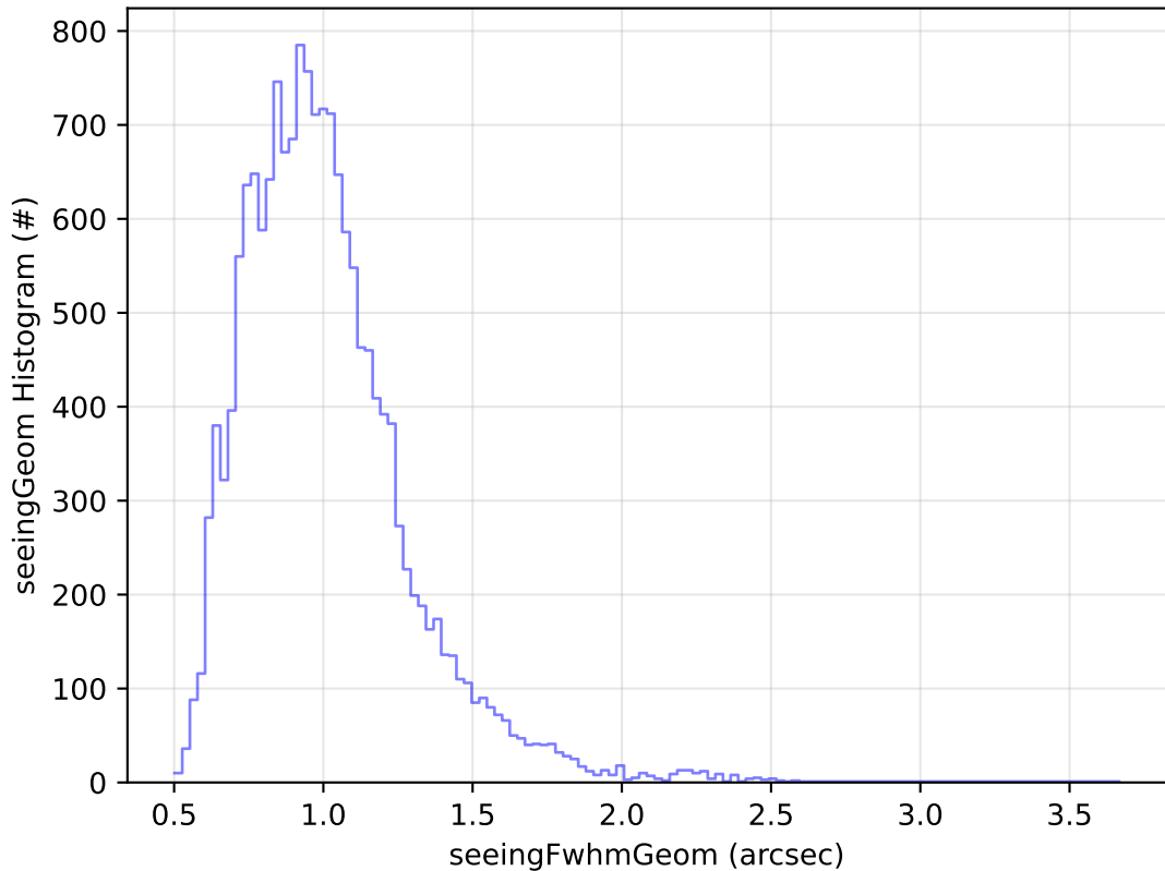
ddf_acor_sf30_lsf40_lsr10_v3.4_10yrs Yr 1 u band: seeingGeom Histogram
