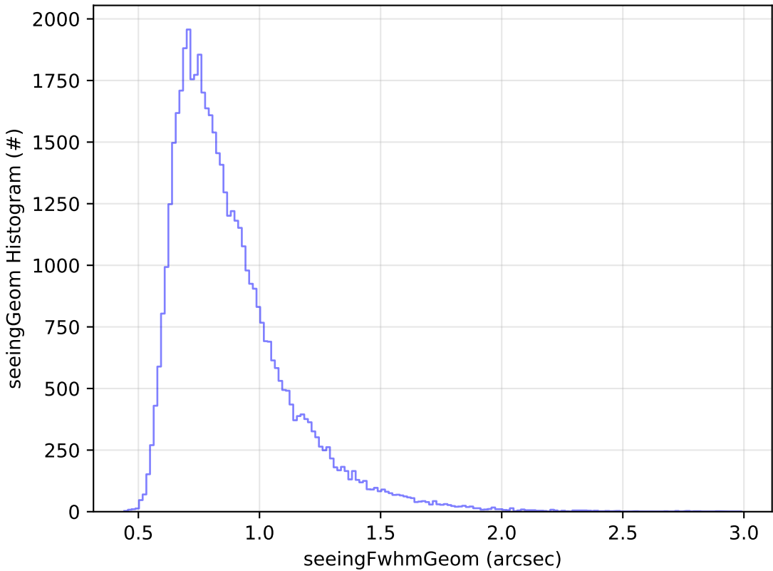
ddf_acor_sf30_lsf40_lsr10_v3.4_10yrs Yr 1 r band: seeingGeom Histogram
