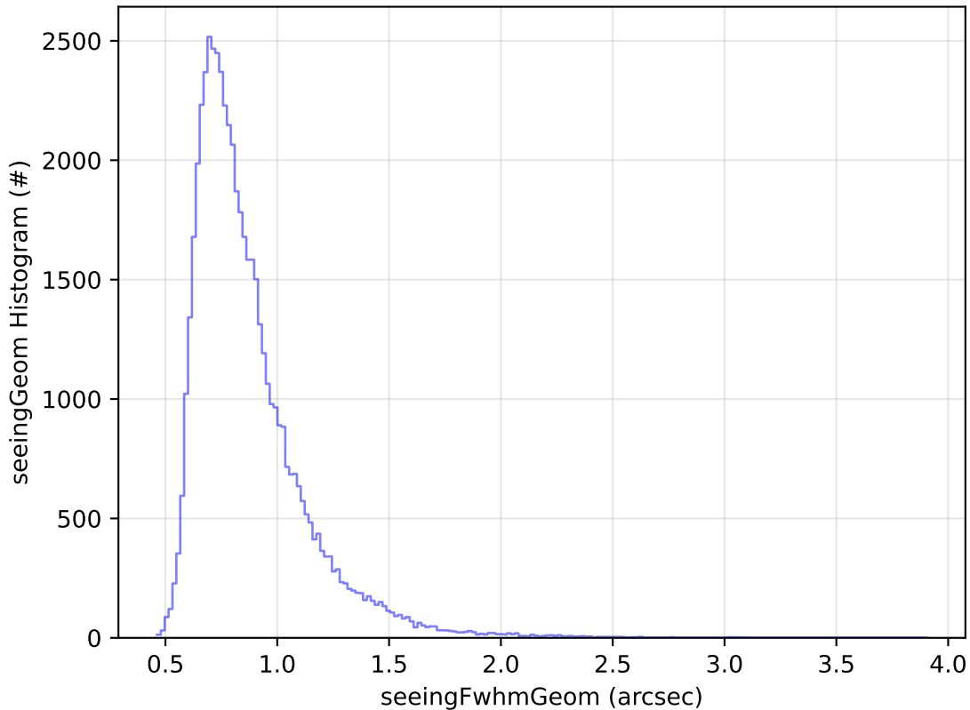
ddf_acor_sf30_lsf40_lsr10_v3.4_10yrs Yr 1 i band: seeingGeom Histogram
