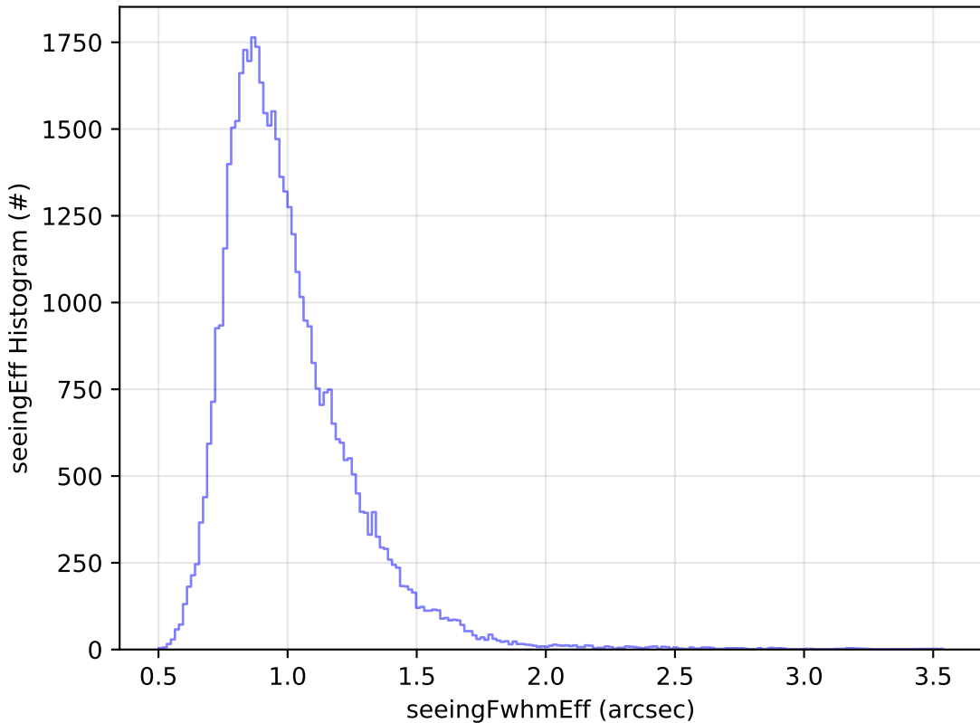
ddf_acor_sf30_lsf40_lsr10_v3.4_10yrs Yr 1 y band: seeingEff Histogram
