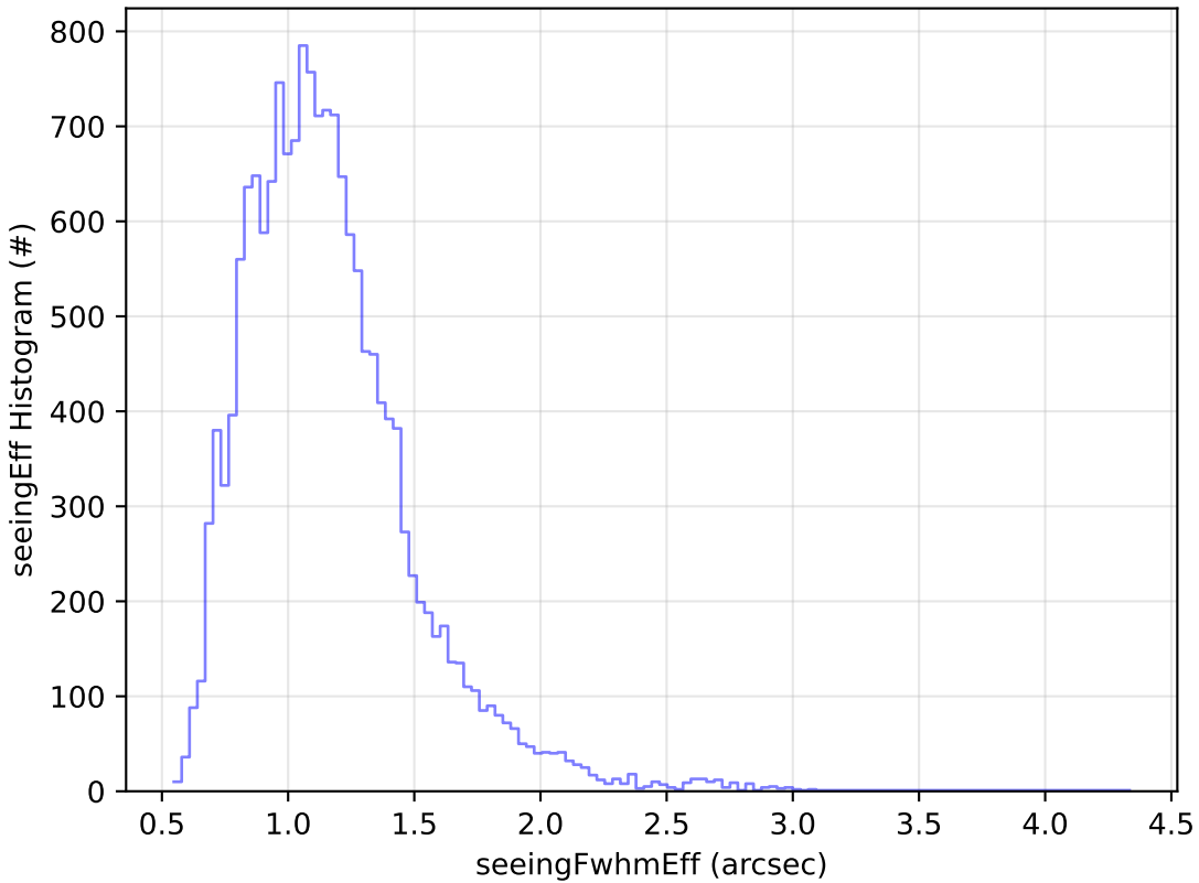
ddf_acor_sf30_lsf40_lsr10_v3.4_10yrs Yr 1 u band: seeingEff Histogram
