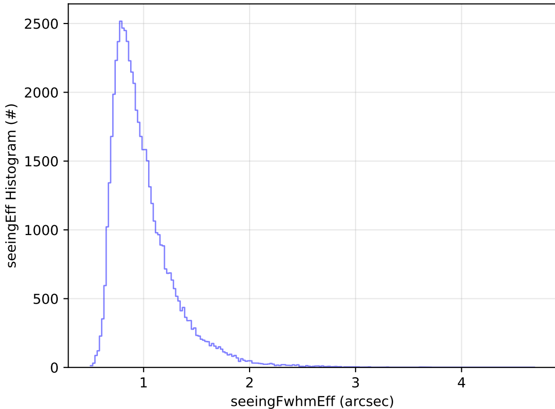
ddf_acor_sf30_lsf40_lsr10_v3.4_10yrs Yr 1 i band: seeingEff Histogram
