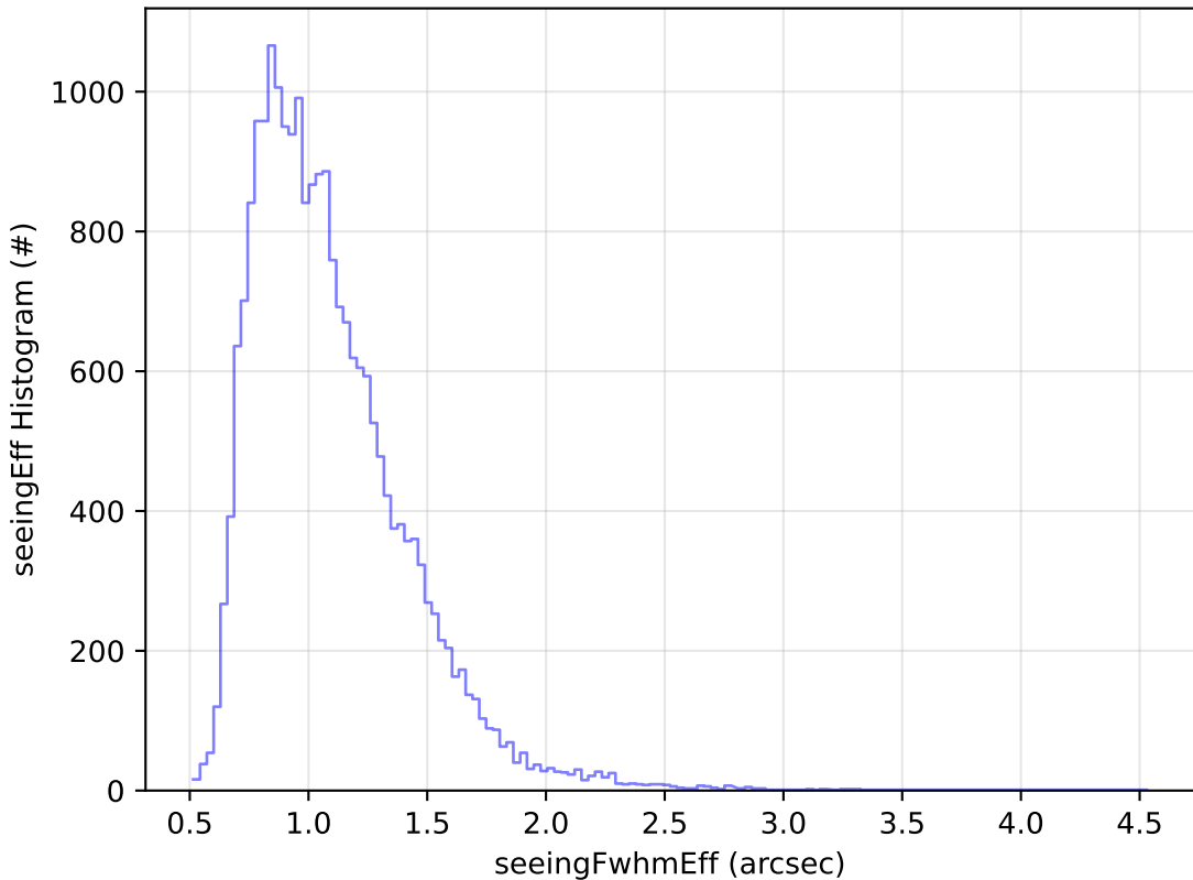
ddf_acor_sf30_lsf40_lsr10_v3.4_10yrs Yr 1 g band: seeingEff Histogram
