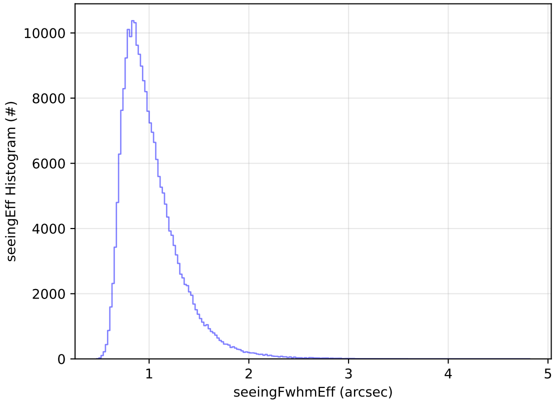
ddf_acor_sf30_Isf40_Isr10_v3.4_10yrs Yr 1 all bands: seeingEff Histogram
