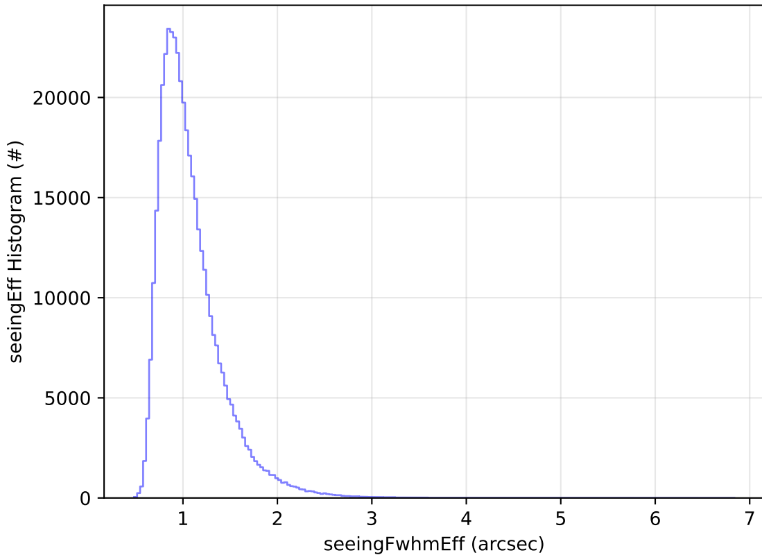
ddf_acor_sf30_lsf40_lsr10_v3.4_10yrs WFD z band: seeingEff Histogram
