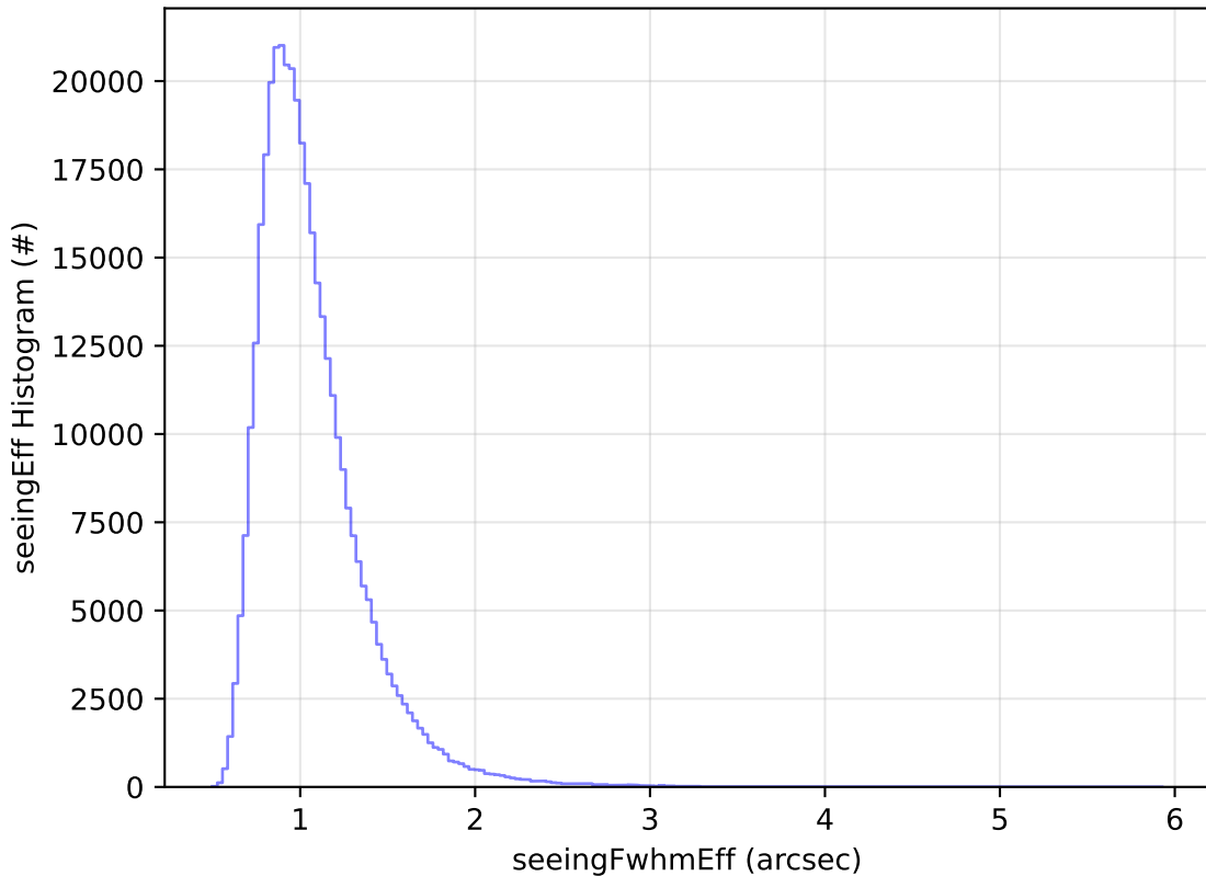
ddf_acor_sf30_lsf40_lsr10_v3.4_10yrs WFD y band: seeingEff Histogram
