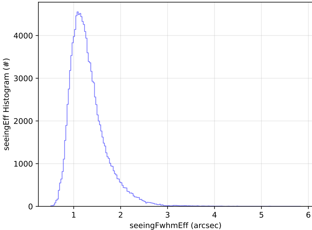
ddf_acor_sf30_lsf40_lsr10_v3.4_10yrs WFD u band: seeingEff Histogram
