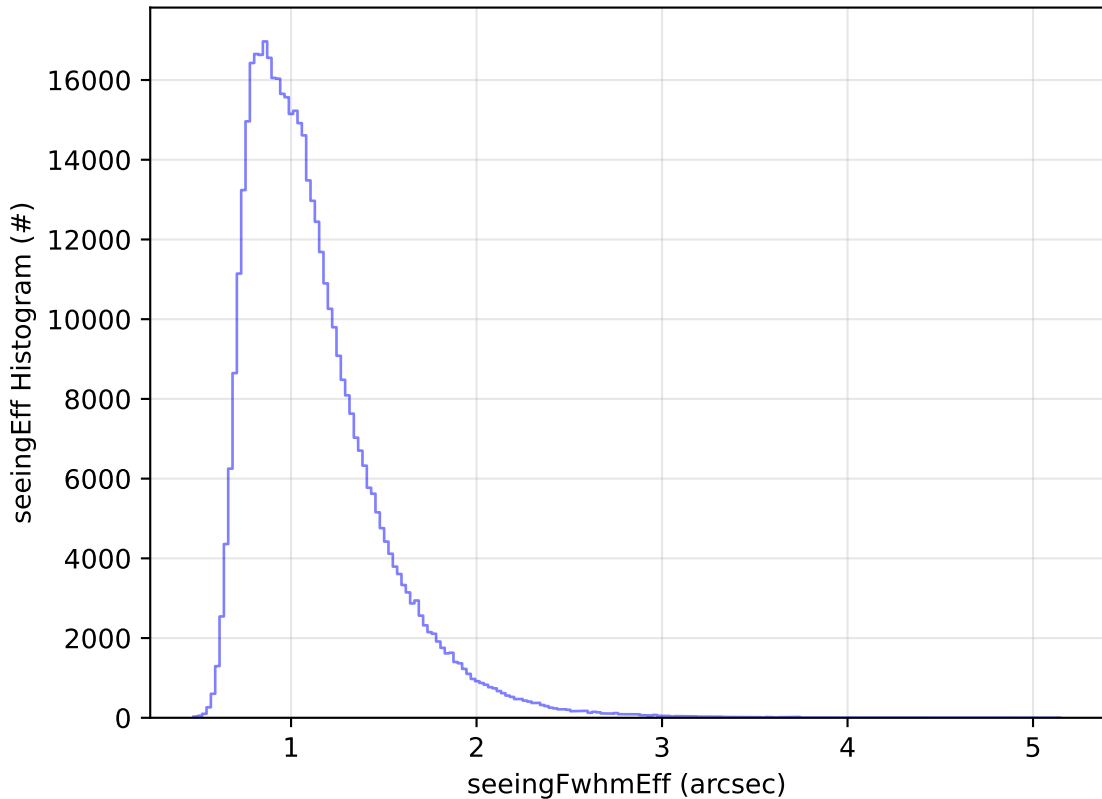
ddf_acor_sf30_lsf40_lsr10_v3.4_10yrs WFD r band: seeingEff Histogram
