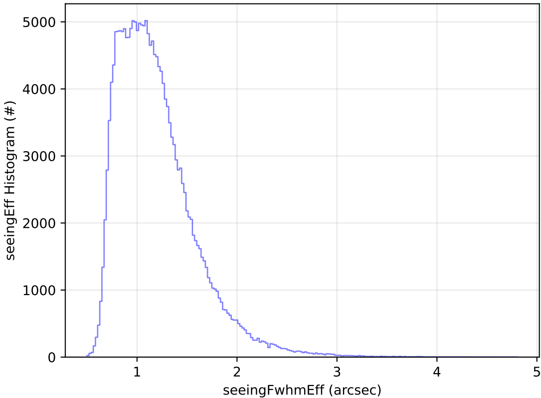
ddf_acor_sf30_lsf40_lsr10_v3.4_10yrs WFD g band: seeingEff Histogram
