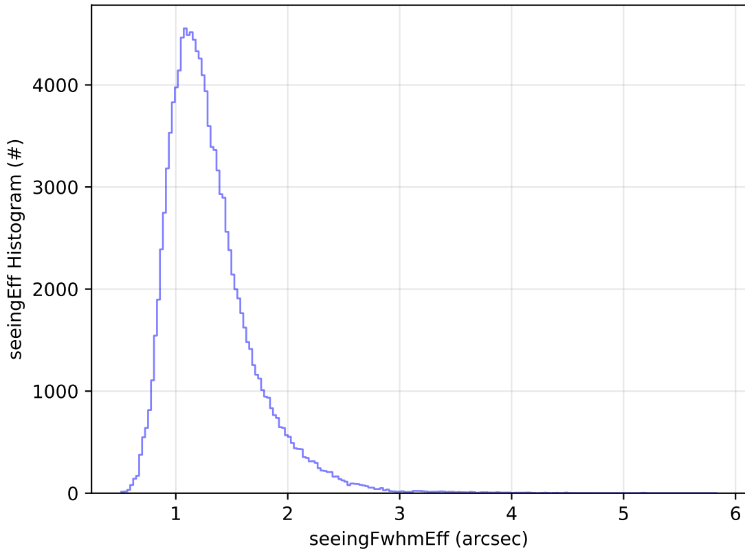
ddf_acor_sf30_ls40_lsr10_v3.4_10yrs All sky u band: seeingEff Histogram
