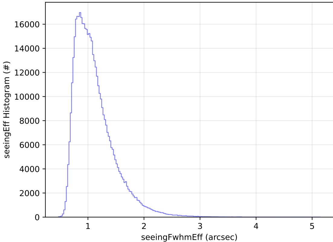
ddf_acor_sf30_lsf40_lsr10_v3.4_10yrs All sky r band: seeingEff Histogram
