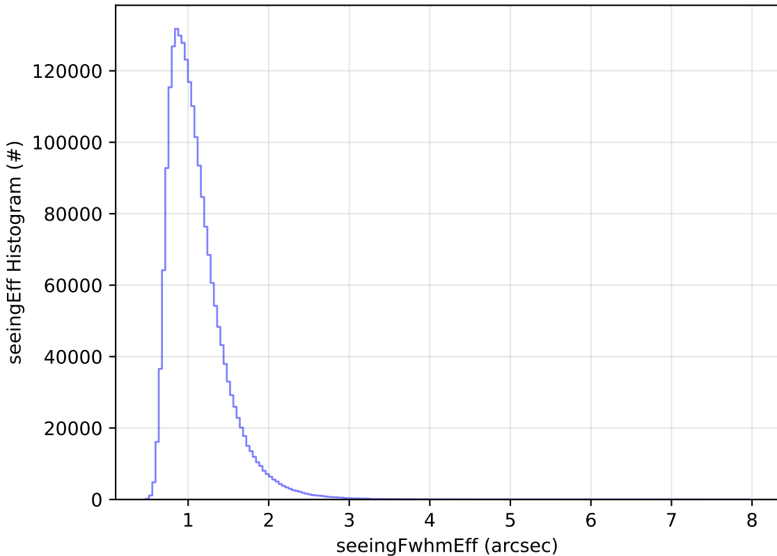
ddf_acor_sf30_lsf40_lsr10_v3.4_10yrs All sky all bands: seeingEff Histogram
