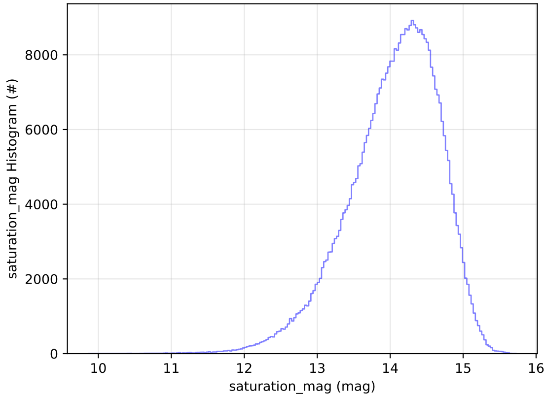
ddf_acor_sf30_lsf40_lsr10_v3.4_10yrs WFD z band: saturation_mag Histogram
