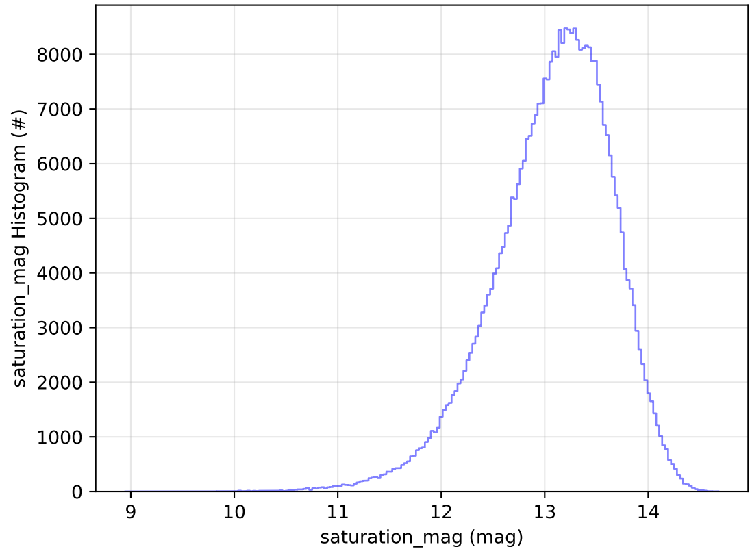
ddf_acor_sf30_lsf40_lsr10_v3.4_10yrs WFD y band: saturation_mag Histogram
