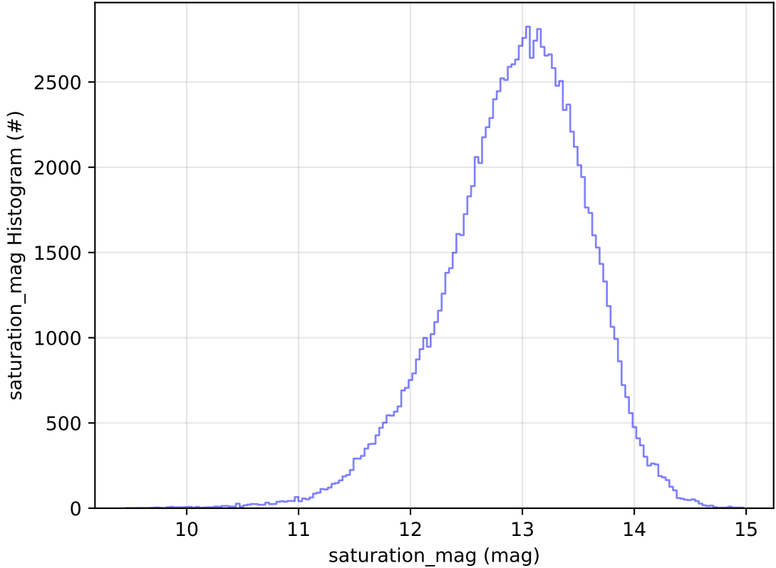
ddf_acor_sf30_lsf40_lsr10_v3.4_10yrs WFD u band: saturation_mag Histogram
