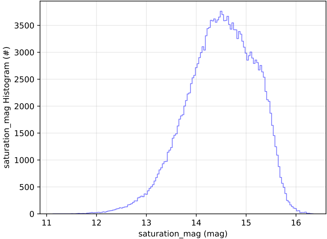
ddf_acor_sf30_lsf40_lsr10_v3.4_10yrs WFD g band: saturation_mag Histogram
