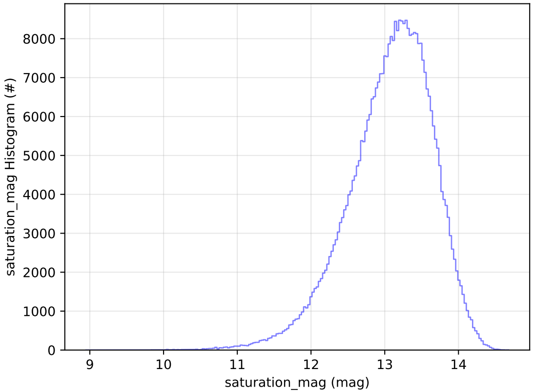
ddf_acor_sf30_lsf40_lsr10_v3.4_10yrs All sky y band: saturation_mag Histogram
