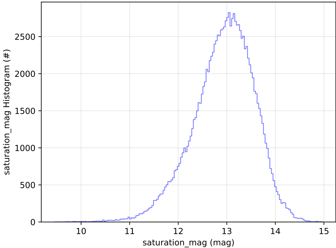
ddf_acor_sf30_lsf40_lsr10_v3.4_10yrs All sky u band: saturation_mag Histogram
