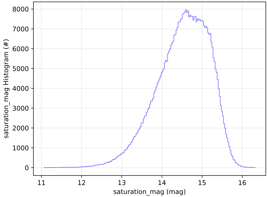
ddf_acor_sf30_lsf40_lsr10_v3.4_10yrs All sky r band: saturation_mag Histogram
