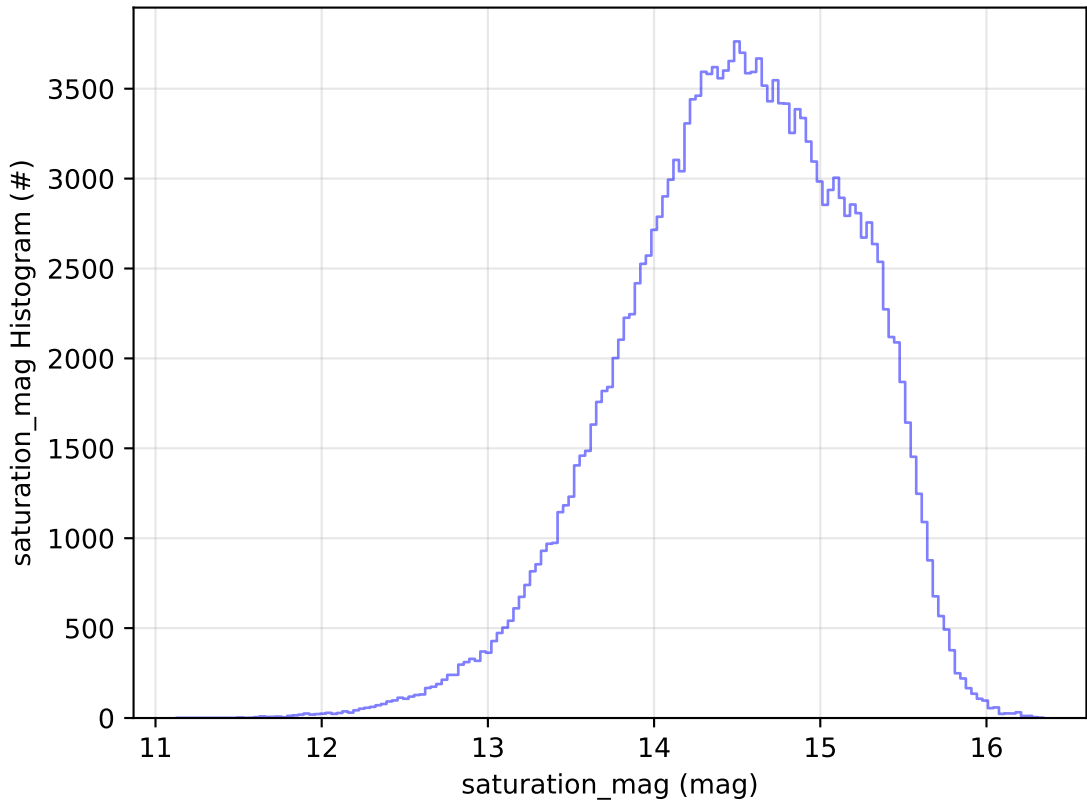
ddf_acor_sf30_lsf40_lsr10_v3.4_10yrs All sky g band: saturation_mag Histogram
