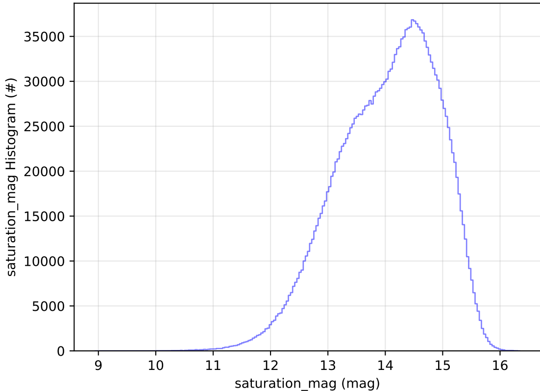
ddf_acor_sf30_lsf40_lsr10_v3.4_10yrs All sky all bands: saturation_mag Histogram
