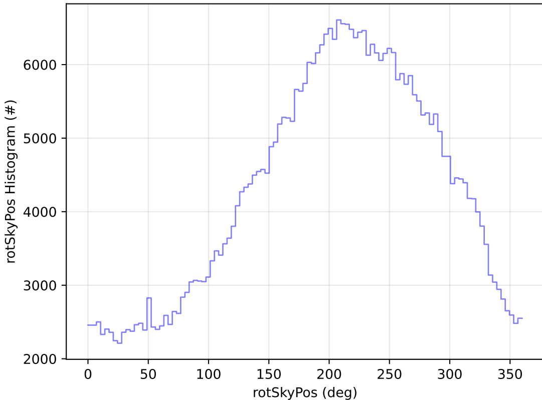
ddf_acor_sf30_lsf40_lsr10_v3.4_10yrs WFD z band: rotSkyPos Histogram
