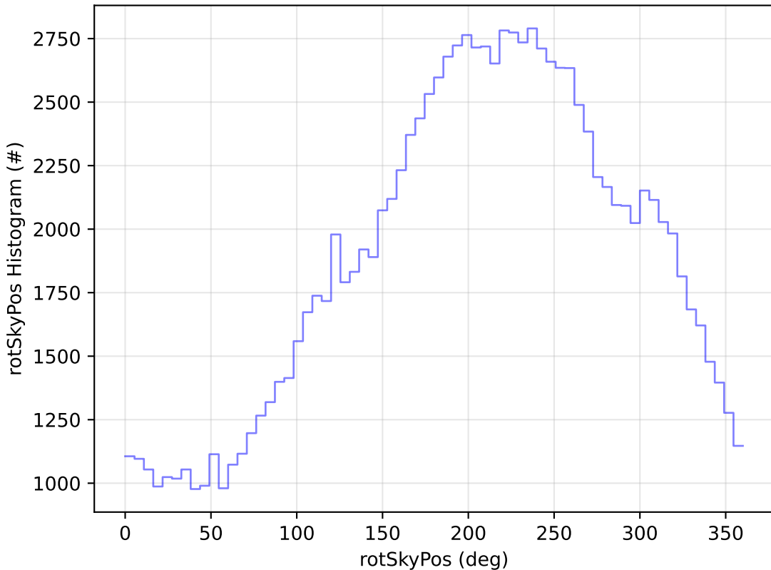
ddf_acor_sf30_lsf40_lsr10_v3.4_10yrs WFD u band: rotSkyPos Histogram
