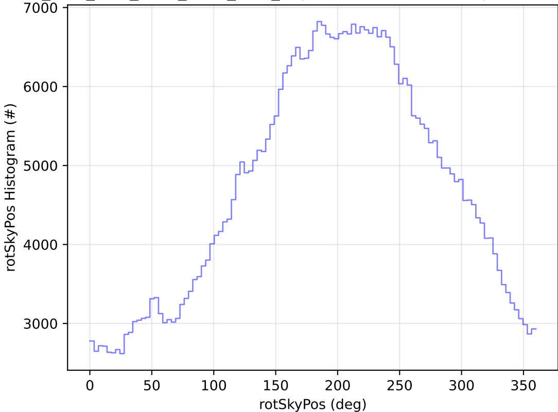
ddf_acor_sf30_lsf40_lsr10_v3.4_10yrs WFD r band: rotSkyPos Histogram
