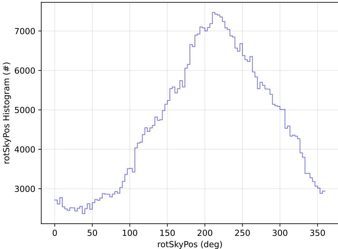
ddf_acor_sf30_lsf40_lsr10_v3.4_10yrs WFD i band: rotSkyPos Histogram
