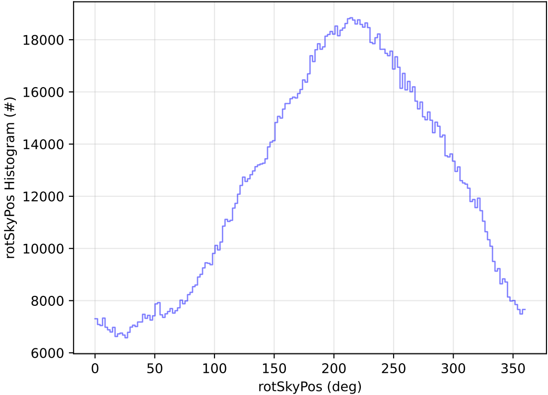
ddf_acor_sf30_lsf40_lsr10_v3.4_10yrs WFD all bands: rotSkyPos Histogram
