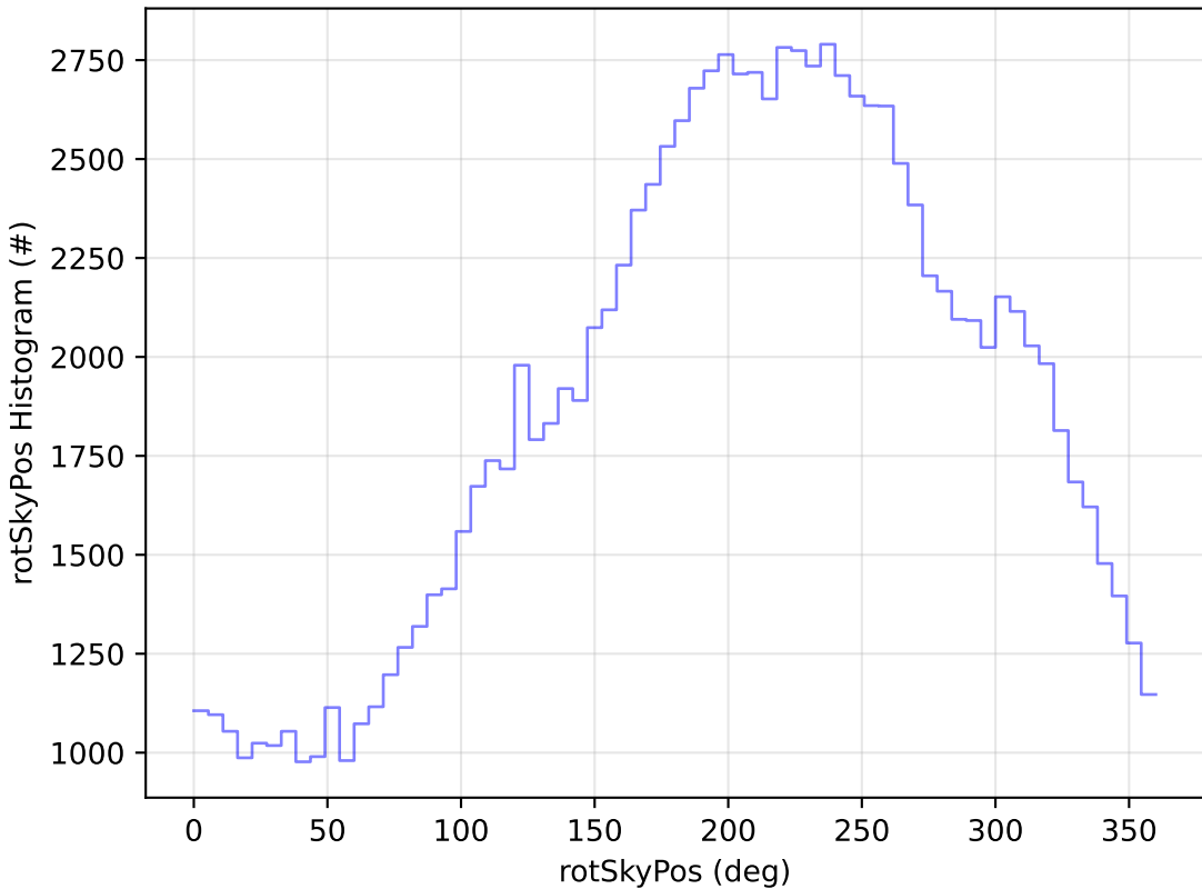
ddf_acor_sf30_lsf40_lsr10_v3.4_10yrs All sky u band: rotSkyPos Histogram
