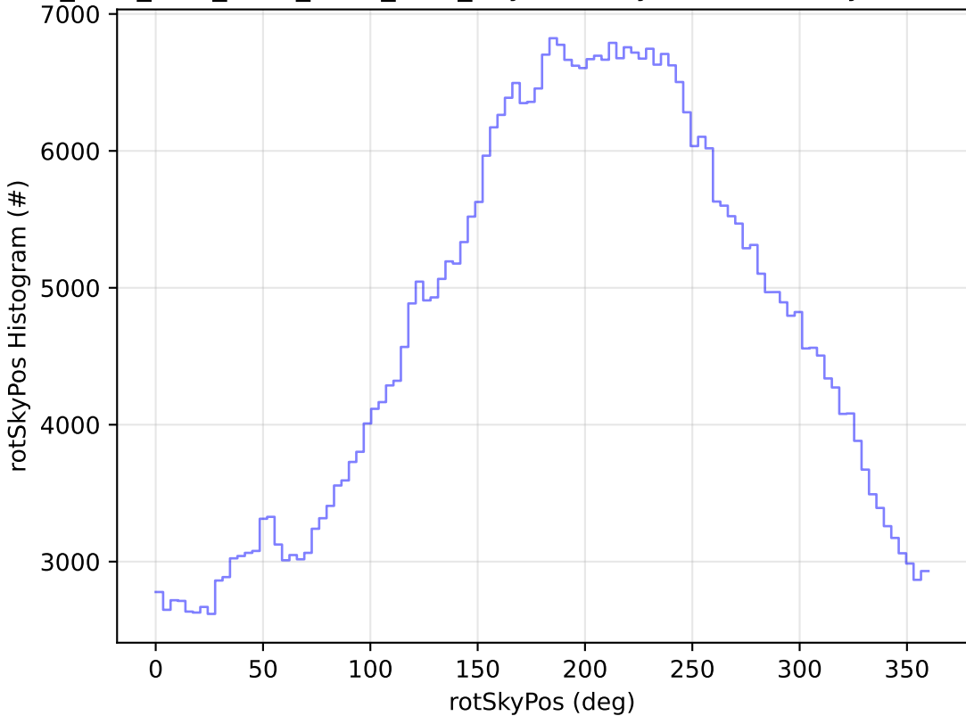
ddf_acor_sf30_ls40_lsr10_v3.4_10yrs All sky r band: rotSkyPos Histogram
