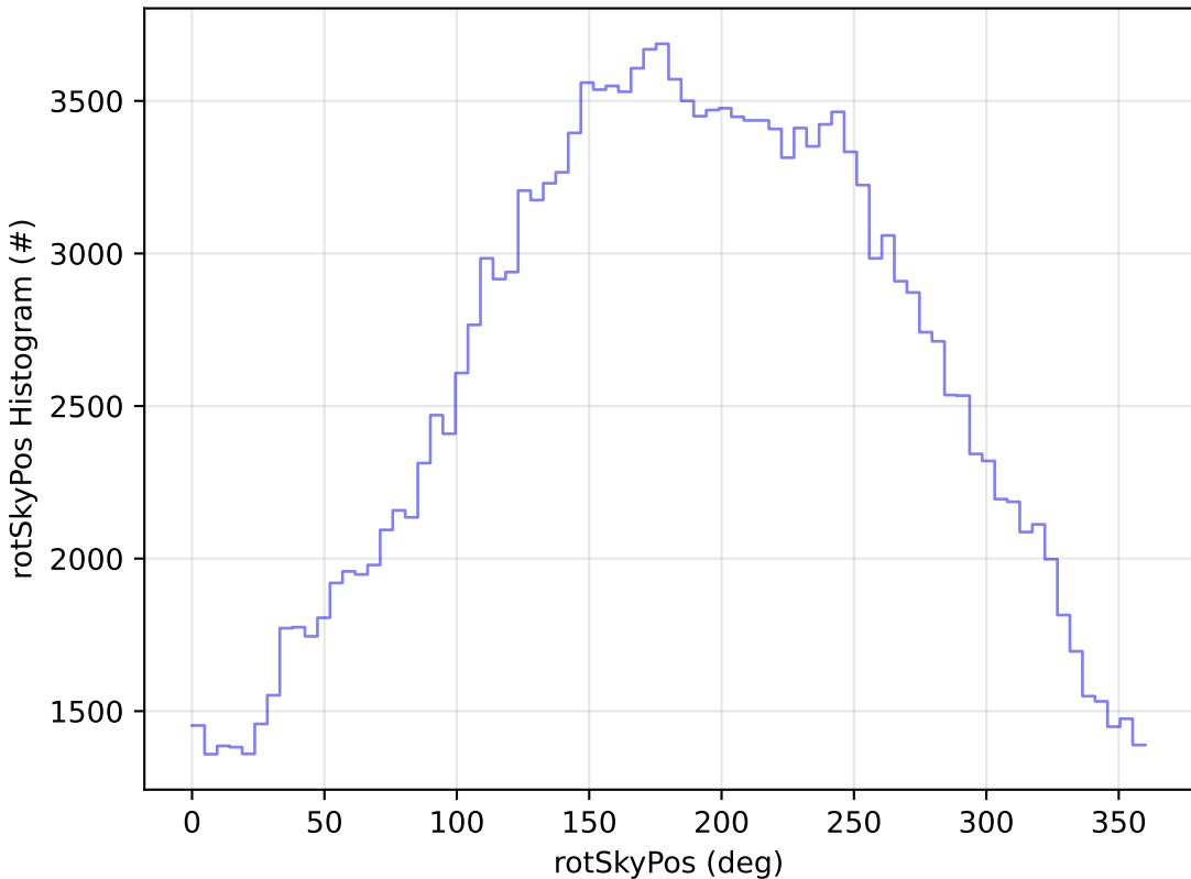
ddf_acor_sf30_lsf40_lsr10_v3.4_10yrs All sky g band: rotSkyPos Histogram
