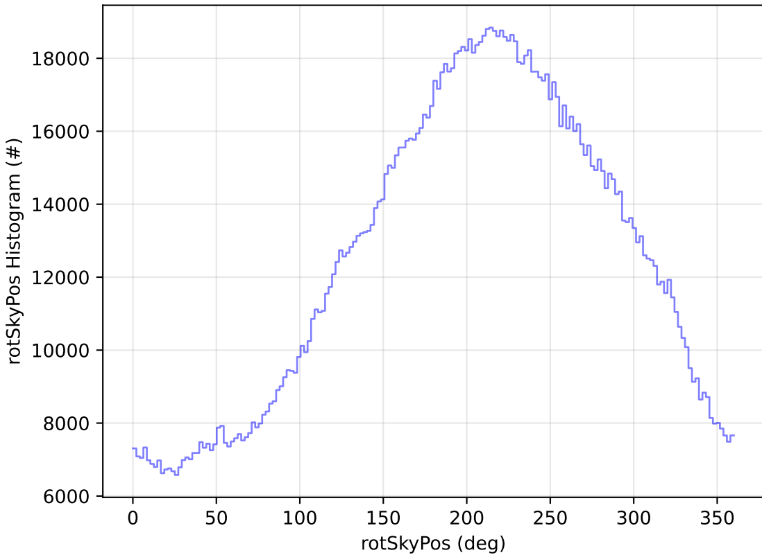
ddf_acor_sf30_lsf40_lsr10_v3.4_10yrs All sky all bands: rotSkyPos Histogram
