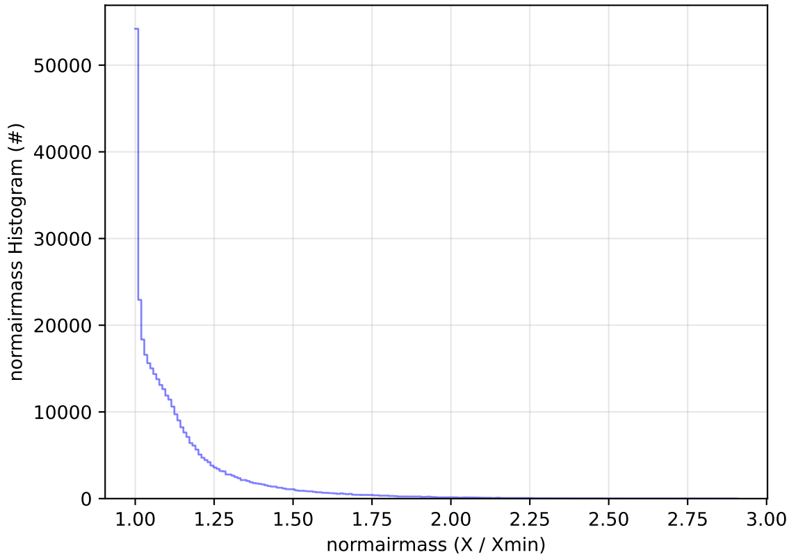
ddf_acor_sf30_lsf40_lsr10_v3.4_10yrs WFD y band: normairmass Histogram
