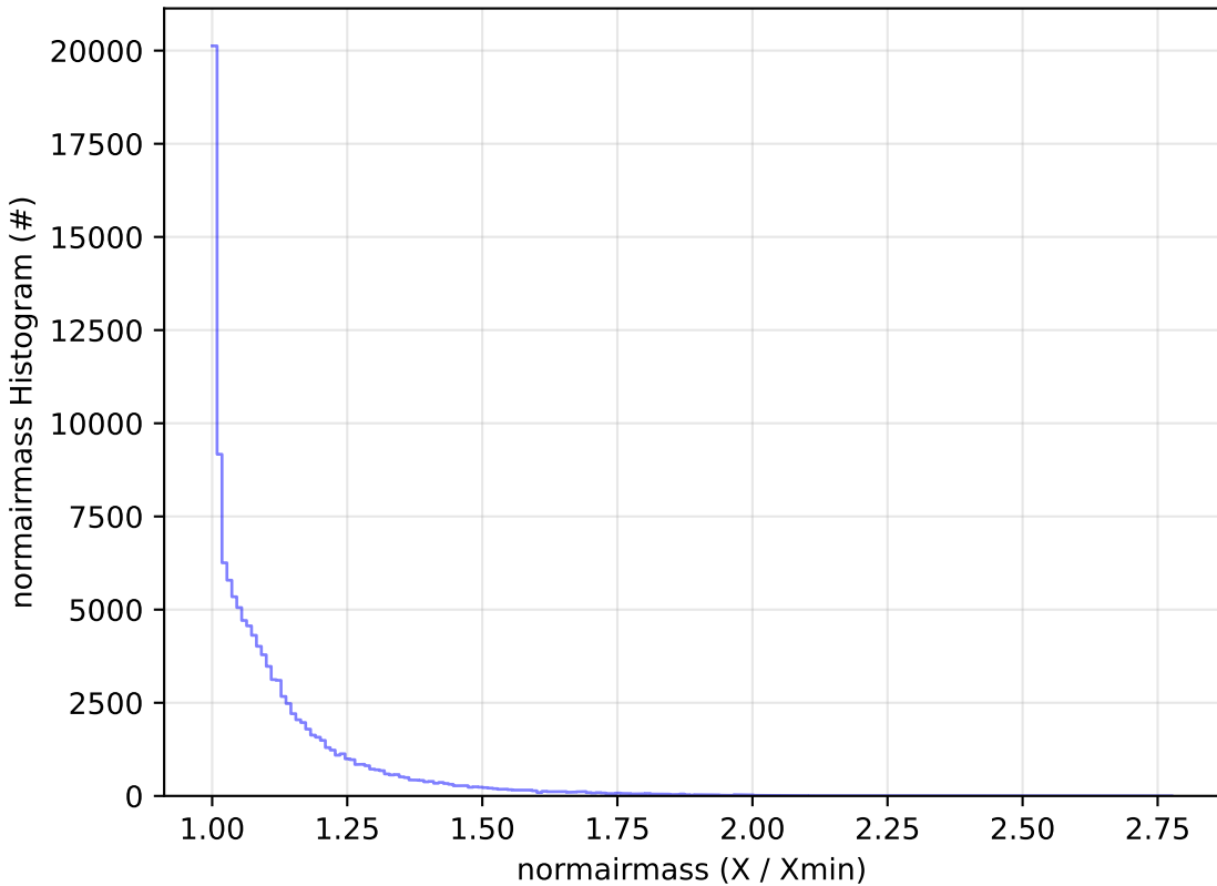
ddf_acor_sf30_lsf40_lsr10_v3.4_10yrs WFD u band: normairmass Histogram
