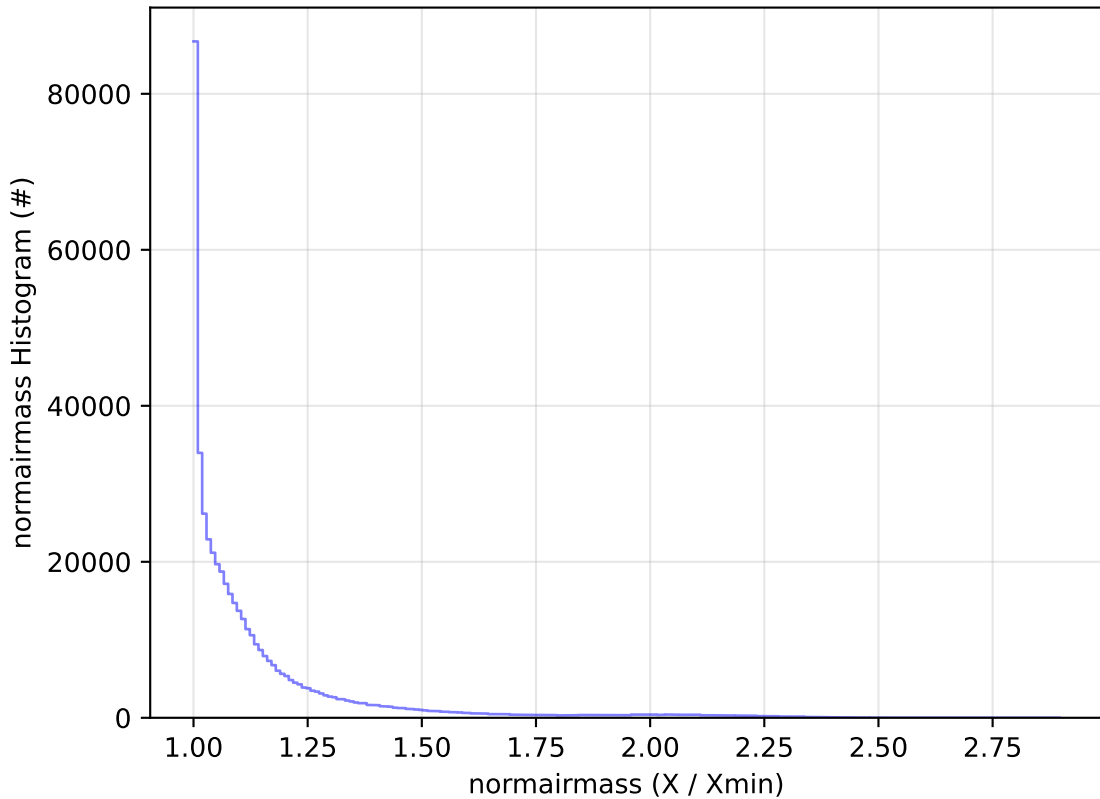
ddf_acor_sf30_lsf40_lsr10_v3.4_10yrs WFD r band: normairmass Histogram
