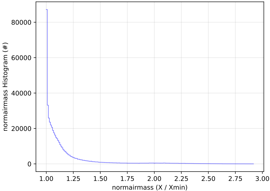
ddf_acor_sf30_lsf40_lsr10_v3.4_10yrs WFD i band: normairmass Histogram
