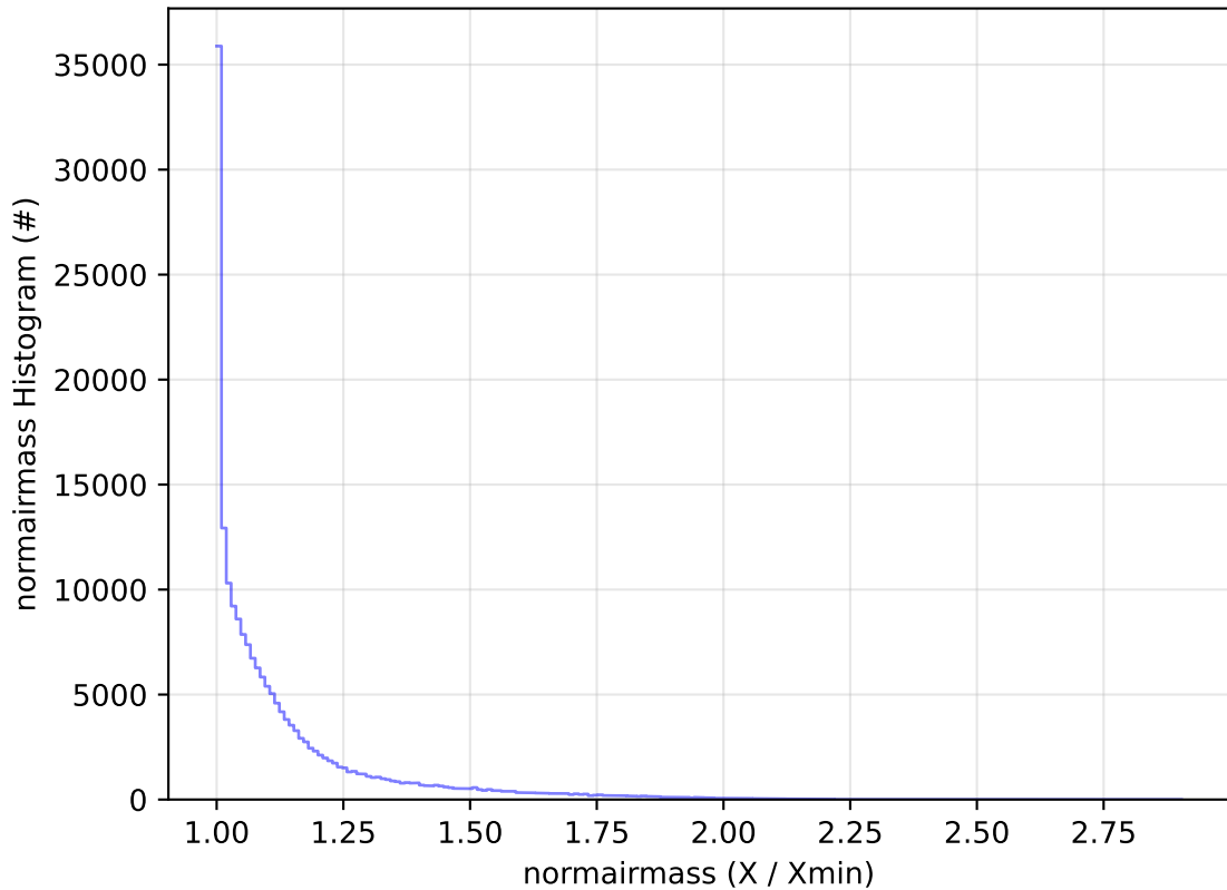
ddf_acor_sf30_lsf40_lsr10_v3.4_10yrs WFD g band: normairmass Histogram
